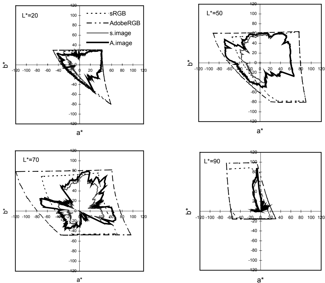
Figure 5 Comparison of gamut boundaries between the source and expanded images of “threads” in linear mapping. The “s.image” represents the source image and “A.image” represents the image mapped into AdobeRGB gamut.
